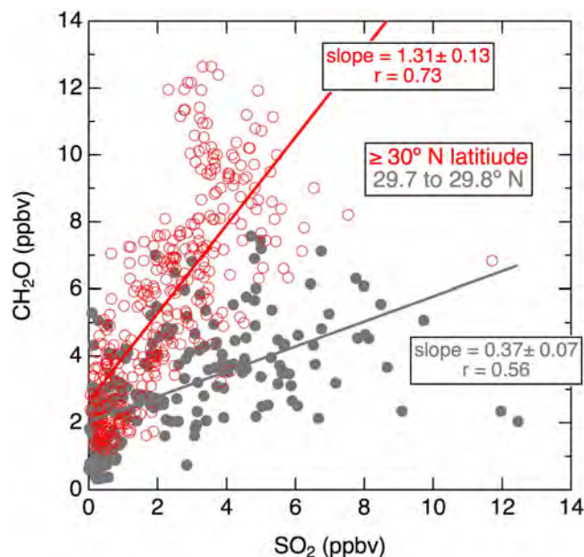
Fig. 8. Relationships between \text{CH}_2\text{O} and \text{SO}_2 measured by the Electra on 27 and 28 August 2000 within the plume from HSC (taken as east of -95.5^\circ longitude to avoid plume from Parish power plant that moves over the western part of the city). The track for the first flight is shown in Fig. 1, and the second flight track was similar. Data are color-coded according to whether they were collected directly over HSC and immediately downwind (grey points, 29.7\text{--}29.8^\circ N) or further downwind (red points, 30.0\text{--}30.3^\circ N). The lines and annotations of the respective colors indicate the linear regressions to the data sets.
