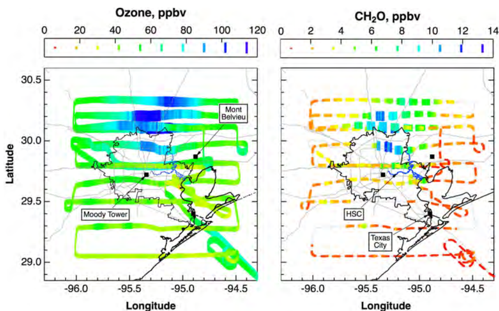
Fig. 1. Distributions of ozone (left) and formaldehyde (right) downwind of the HSC measured by the Electra aircraft during TexAQ5 2000. The data were collected between 12:00 and 18:00 local standard time, and are plotted on the 27 August 2000 flight track, with the symbols sized and color-coded according to the measured mixing ratios of the respective species as indicated by the keys above each plot. During this flight, measured winds were southerly (wind direction = 162 \pm 17^\circ ) and steady (wind speed = 5.4 \pm 1.5 \text{ m s}^{-1} ), where standard deviations of the respective quantities are indicated. Text boxes with arrows indicate approximate locations of specific petrochemical complexes and a measurement site referred to in the text.
